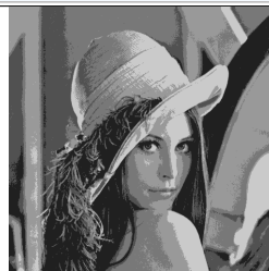
K-means quantization
